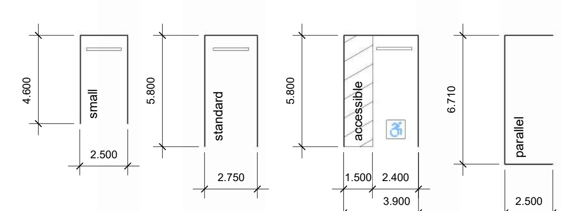
2 Vehicle Parking Stalls SCALE: N.T.S.
